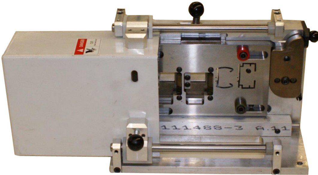
1" VENETIAN CUTTER
