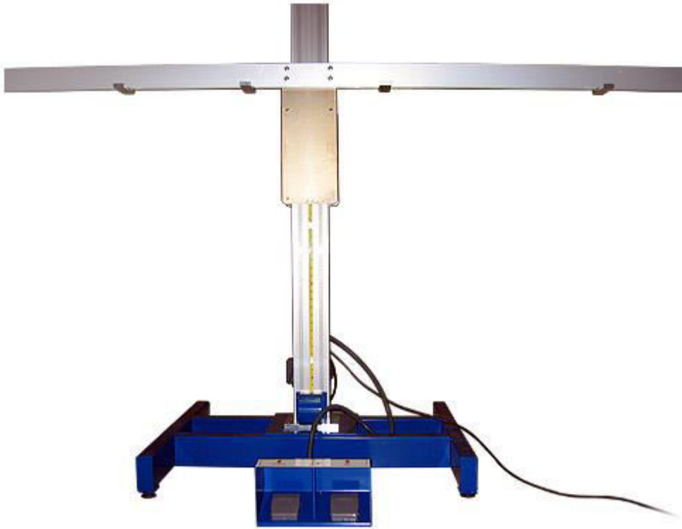
INSPECTION HOIST
