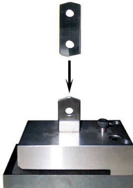
PUNCH AND DIE SET
